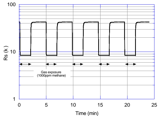
Fig. 10 - Repeatability
