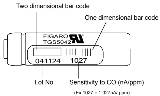
Figure 23 - TGS5042 markings
